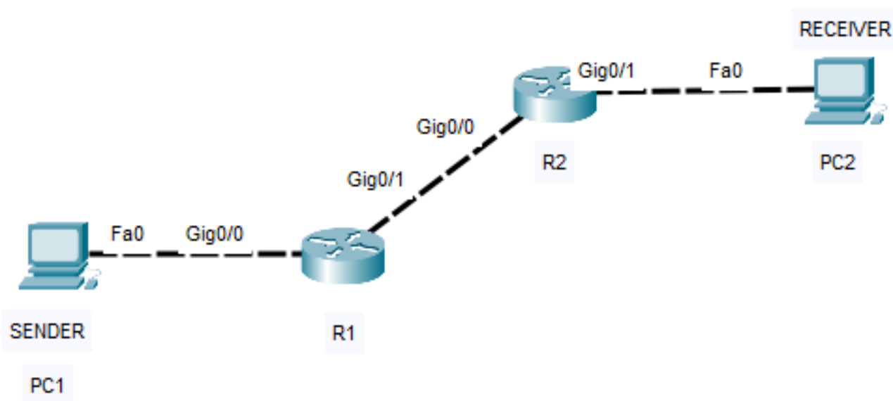
Figure 1: Physical Topology
